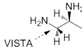
(S)-1,2-diaminopropano
